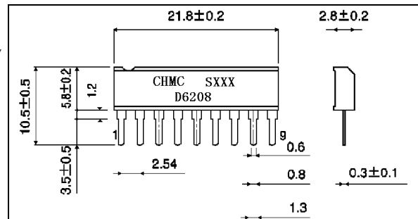
Outline Drawing
